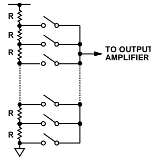
Figure 31. Resistor String
