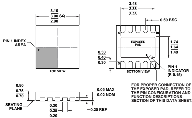
Figure 46. 10-Lead Lead Frame Chip Scale Package [LFCSP] 3 mm × 3 mm Body and 0.75 mm Package Height (CP-10-9)
